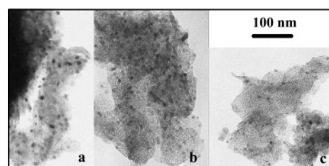
Figure 6. TEM images after treatment at 723 K of (a) Ni 1.4 -Mg/Al under air flow, (b) Ni 1.4 -Mg/Al under N 2 flow and then reduced at 873 K.
